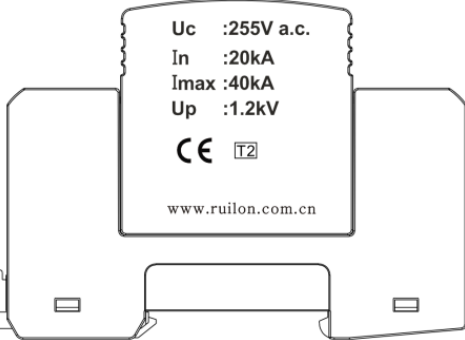
TA40-255N 标识 Marking
